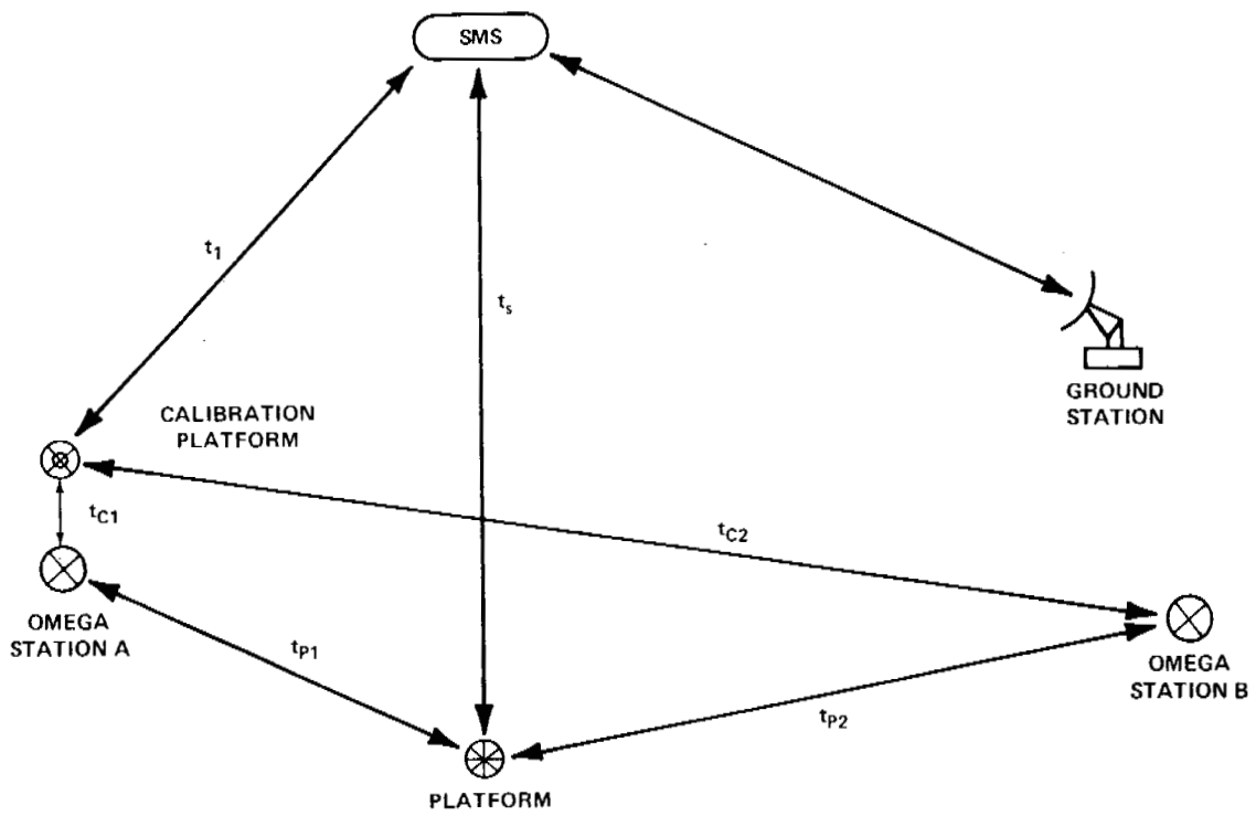
Figure 4. Time-of-arrival technique.
